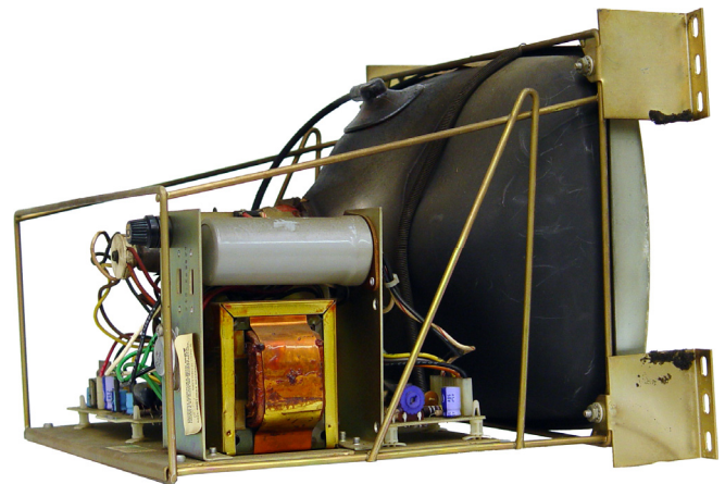
Original Ball Brothers TV-12 CRT Monitor
